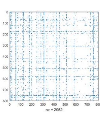
(a) Adjacency matrix
