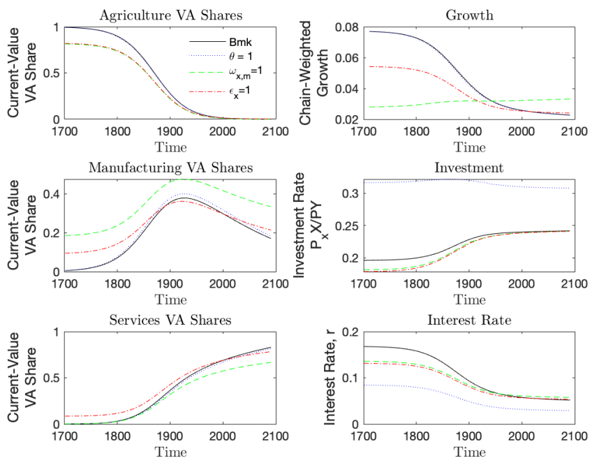
Figure 5: Alternative Models
