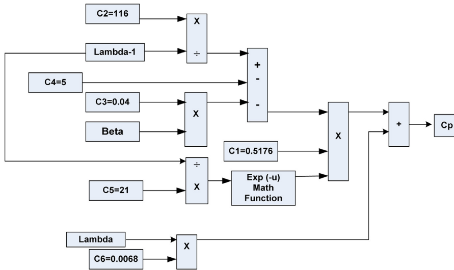
Fig. 4. The simulation block diagram for the calculation of C_p .
