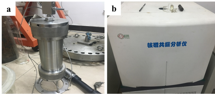
Fig. 12. Main test instruments of imbibition experiment (a-imbibition vessel; b-nuclear magnetic resonance instrument).
