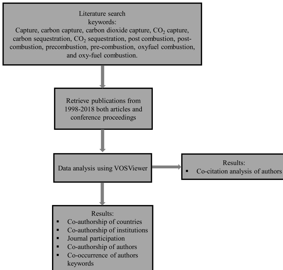
Fig. 1. Methodology flowchart.
