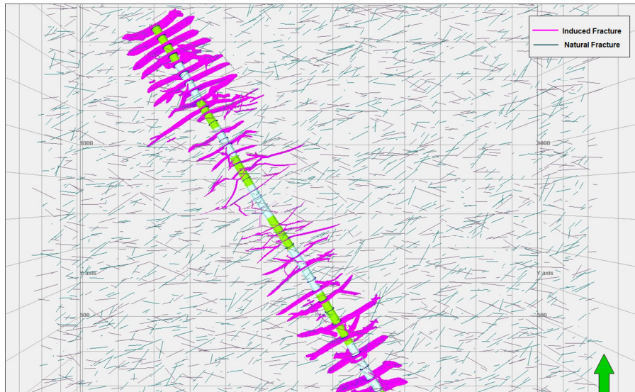
Fig. 3. Simplistic representation of constructed model.
