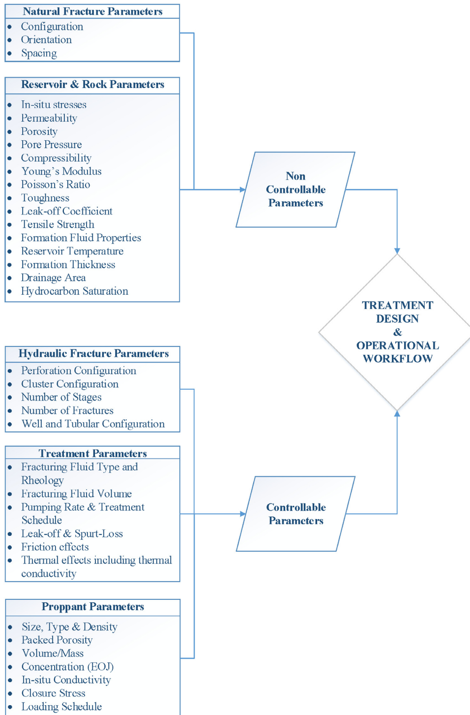
Fig. 4. Parameters incorporated for proposed workflow - Fracturing.
