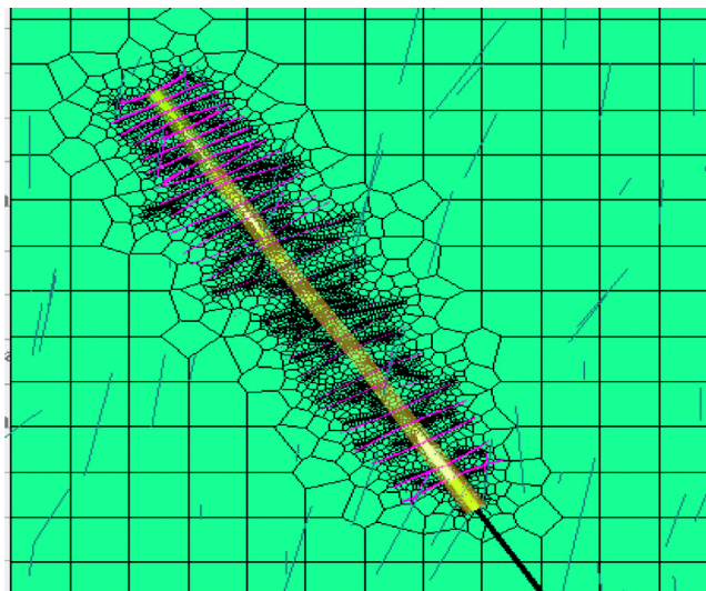
Fig. 7. Extended model — Pressure distribution [View B].
