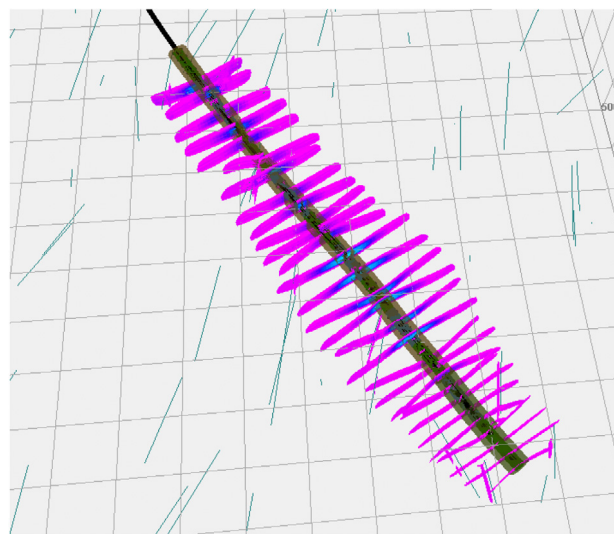
Fig. 6. Extended model — Fracture propagation [View A].
