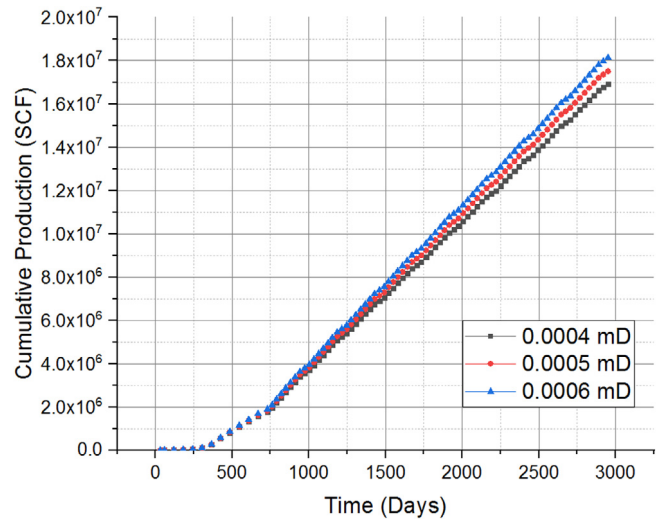
Fig. 15. Change in production w.r.t. permeability.
