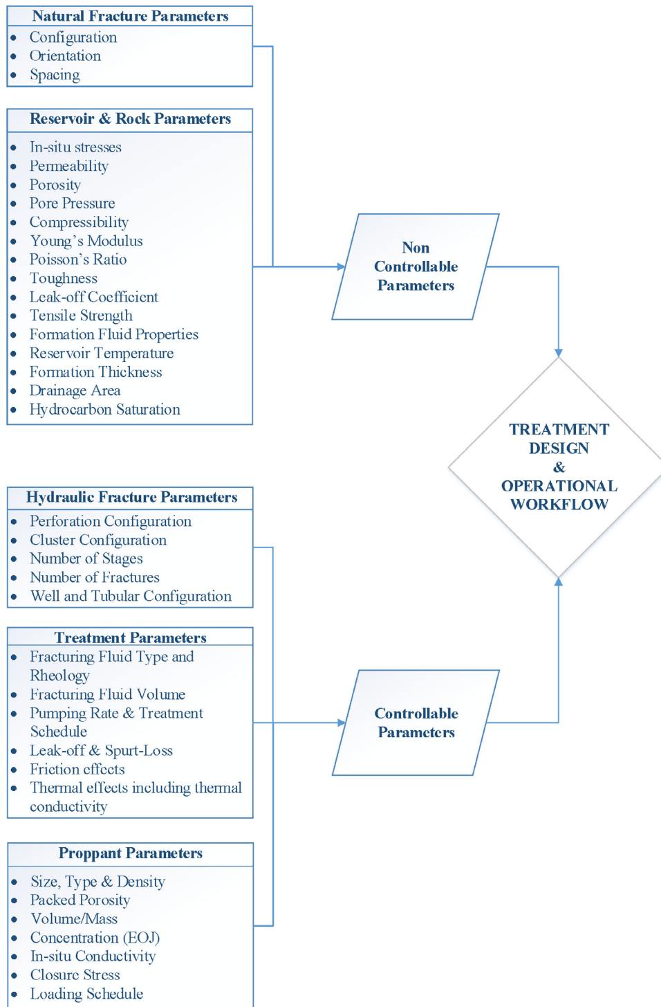
Fig. 4. Parameters incorporated for proposed workflow – Fracturing.
