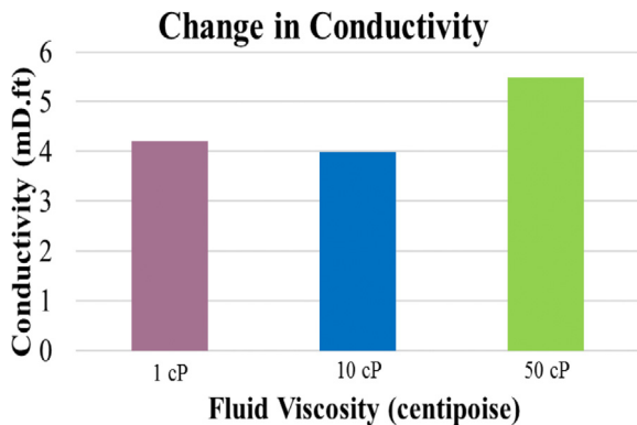
Fig. 14. Change in fracture conductivity w.r.t. fluid viscosity.
