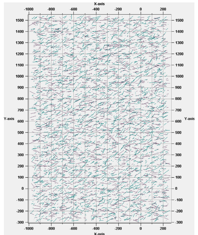
Fig. 11. 2D Discrete Fracture Network (DFN) with multiple orientation – Realistic model.
