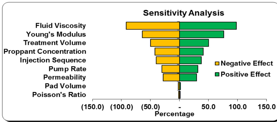
Fig. 17. Sensitivity analysis on design parameter conducted.
