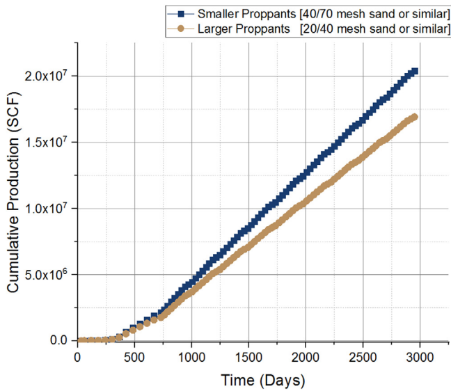
Fig. 12. Change in production w.r.t. proppant size – Single Proppant Injection.
