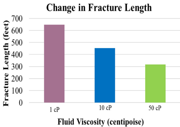
Fig. 13. Change in fracture length w.r.t. fluid viscosity.
