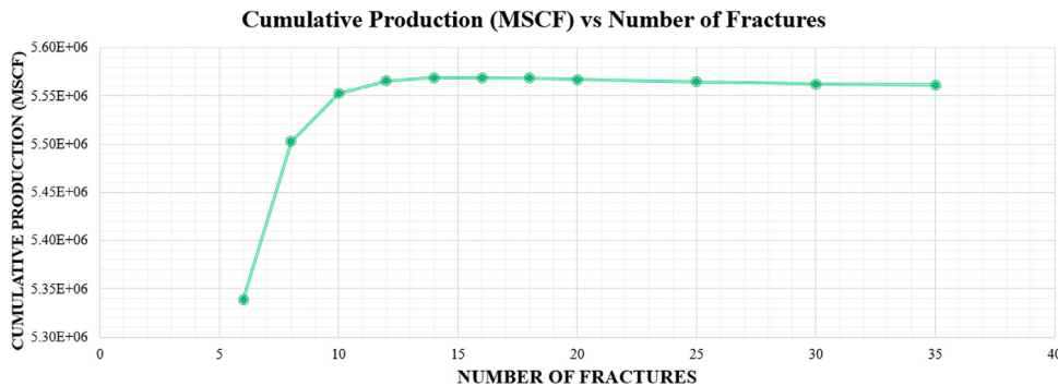
Fig. 19. Cumulative production with respect to number of transverse fracture.
