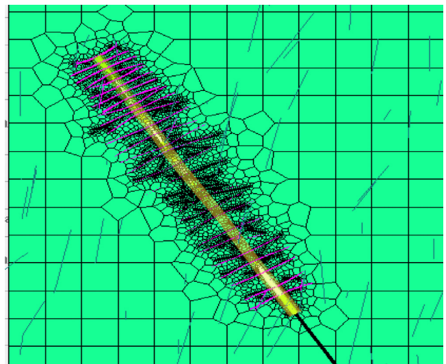
Fig. 7. Extended model – Pressure distribution [View B].
