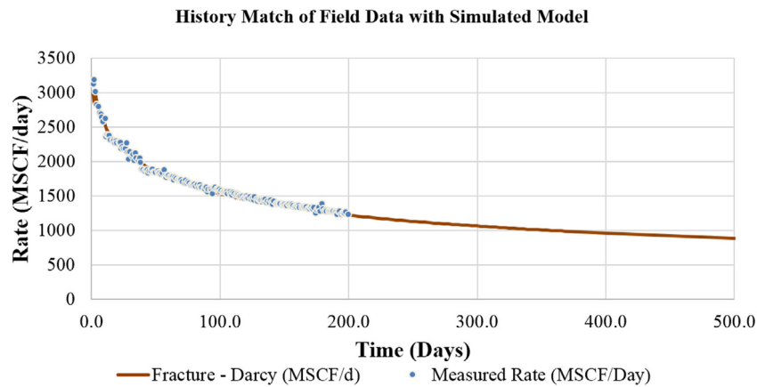
Fig. 5. History matching of constructed model.
