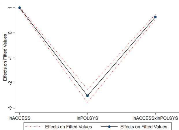
Fig. 5. Income inequality model verification. NB: The red short-dash dot-dot represents the Conditional Marginal Effects with 95% CIs.
