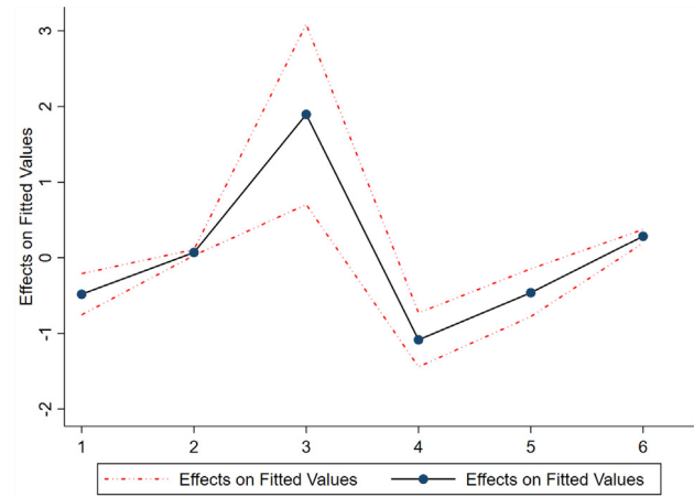
Fig. 7. Human development index model verification. NB: The red short-dash dot-dot represents the Conditional Marginal Effects with 95% CIs. Here, 1 is lnGINI_DIS, 2 is lnACCESS, 3 is lnPOLSYS, 4 is lnACCESSxlnPOLSYS, 5 is lnGINI_DISxlnPOLSYS, and 6 represents lnACCESSxlnPOLSYSxlnGINI_DIS.
