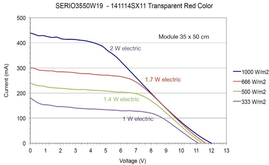
Fig. 9. The DSSC electrical characteristic for Module SERIO3550W19.. (For interpretation of the references to color in this figure legend, the reader is referred to the web version of this article.)
