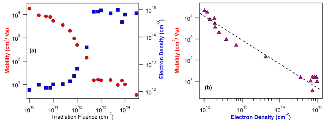
Fig. 7. (a) Mobility (red circles) and electron density (blue squares) as a function of irradiation fluence for InSb-MBE films irradiated with 17 MeV Au +7 ions. (b) Mobility as a function of electron density for the same samples shown in (a).
