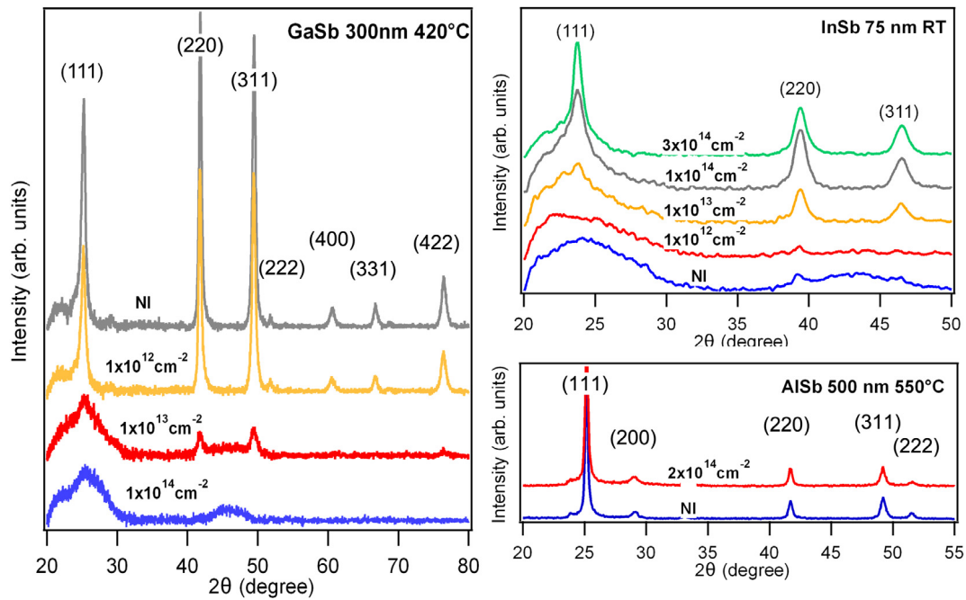
Fig. 5. GIXRD of GaSb-sputt, InSb-sputt (75 nm) and AlSb-sputt films as deposited and after irradiation with 17 MeV Au +7 ions. Diffractograms from samples irradiated with different fluences are vertically offset for clarity.
