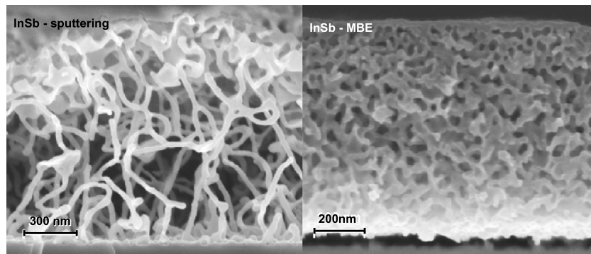
Fig. 3. SEM micrographs of InSb-sput and InSb-MBE films, after irradiation with 17 MeV Au +7 ions to a total fluence of 2 \times 10^{14} \text{ cm}^{-2} . The thicknesses of the unirradiated films were 75 nm (InSb-sputt) and 370 nm (InSb-MBE), respectively.
