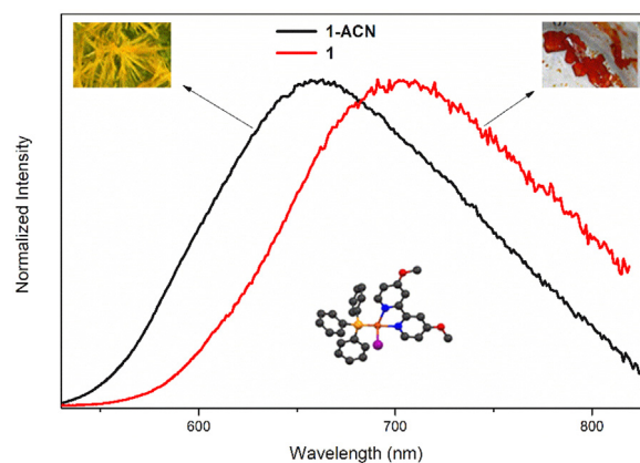
Fig. 3. Normalized PL spectra ( \lambda_{exc} = 420 nm) for powders of 1 = CuI(PPh 3 )(L) (red curve) and 1-ACN (black curve) at room temperature. Detail: photograph of the orange (right) and yellow (left) compounds. (For interpretation of the references to colour in this figure legend, the reader is referred to the web version of this article.)
