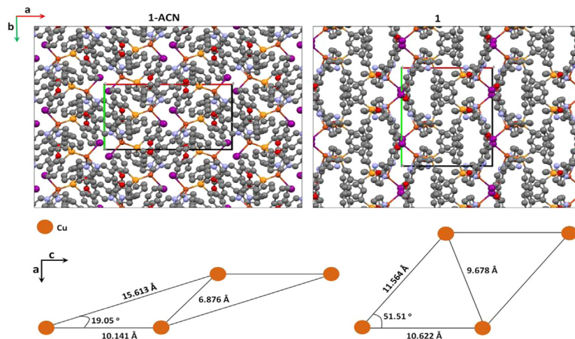
Fig. 4. 2D visualization of the molecular packing for compound 1-ACN (left) and 1 (right). The atoms Cu, N, P, O, I, C are represented by the orange, blue, yellow, red, violet and gray colors, respectively. Hydrogen atoms were left out for better visualization of the molecular packaging. (For interpretation of the references to colour in this figure legend, the reader is referred to the web version of this article.)
