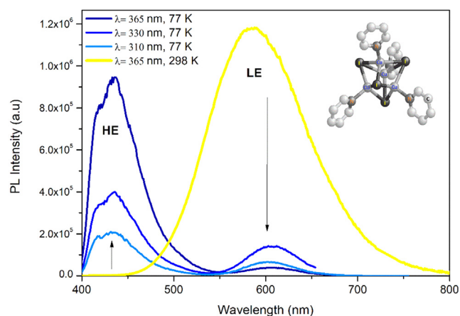
Fig. 6. PL spectra ( \lambda_{exc} = 310, 330 e 365 nm) at 77 K and 298 K ( \lambda_{exc} = 365 nm) for Cu_4I_4py_4 powder sample.
