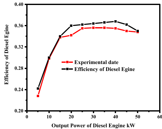
Fig. 2. Change of diesel engine efficiency with output power.
