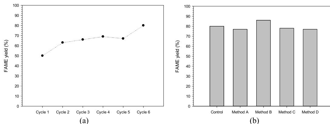
Fig. 3. (a) FAME yield of the consecutive cycles under batch regime (control). (b) FAME yield attained (6th operation cycle) for each enzyme regeneration method. Conditions: 50 °C, 8 h, MeOH/oily mixture = 4:1 (mol/mol), enzyme loading 10% wt.
