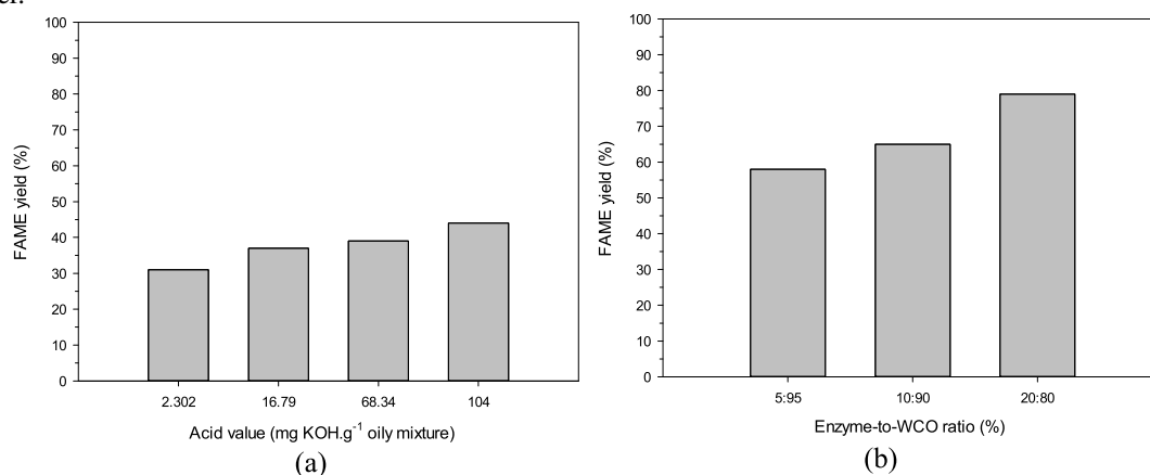
Fig. 2. FAME yield as function of (a) acidity, from different oily mixtures; and (b) enzyme-to-WCO ratio. Conditions: 50 °C, 8 h, MeOH/oily mixture = 4:1 (mol/mol), acid value of 104 mg KOH g -1 .
