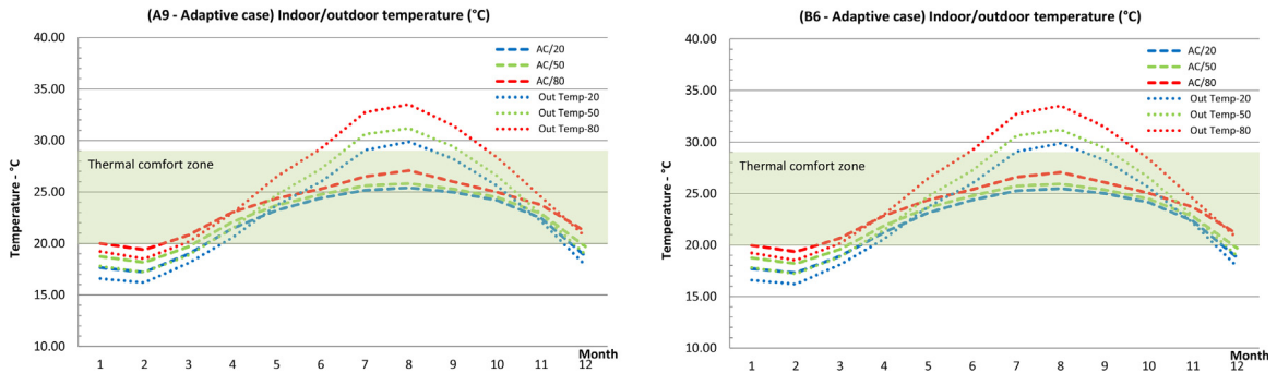
Fig. 6. Temperature and thermal comfort indications for the adaptive case (AC).
