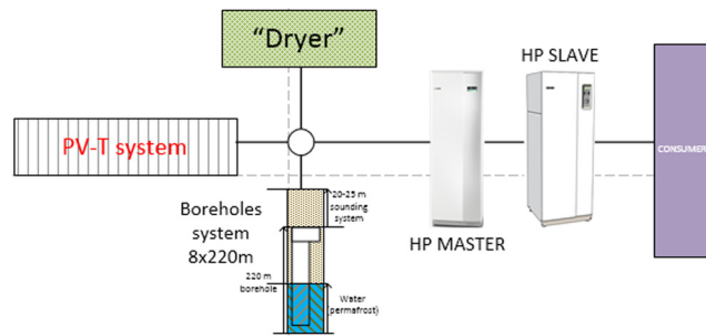
Fig. 1. Installation diagram.
