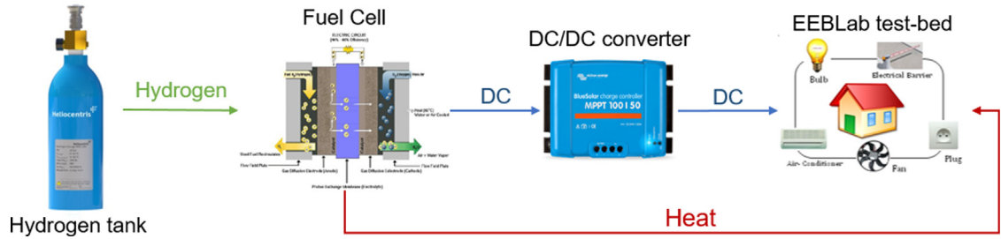
Fig. 1. System's architecture.
