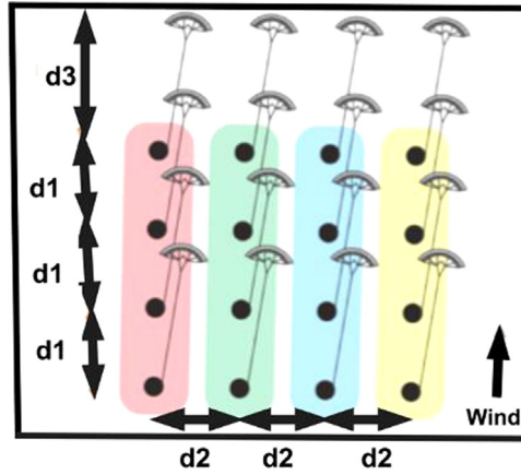
Fig. 1. Layout of wind farm.
