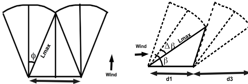
Fig. 2. Minimum distance between two units.
