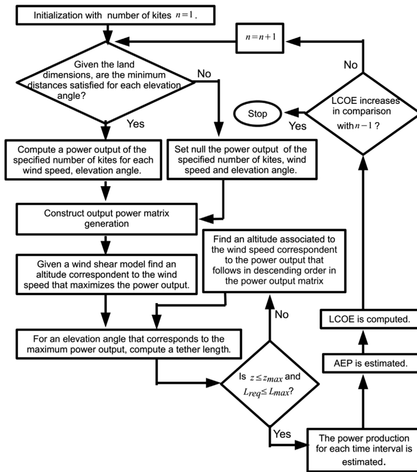
Fig. 3. Algorithm flowchart.
