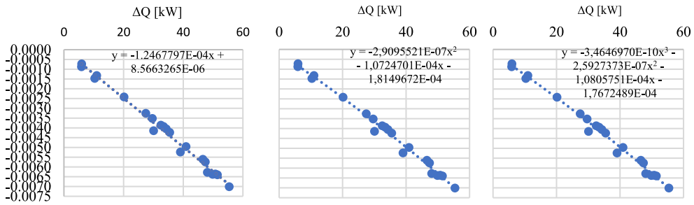
Fig. 4. Linear, quadratic and cubic interpolations of MT user type with their respective equations.
