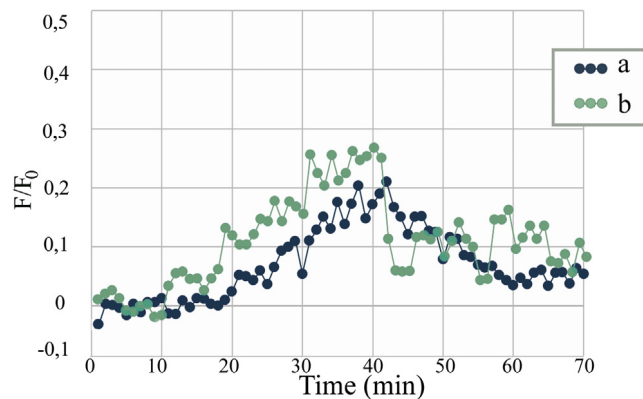
Fig. 4. ROS signals detected in hippocampal CA3 area, with the ROS indicator H 2 DCFDA, corrected for autofluorescence. In the first 10 min the brain slices were in ACSF. From the 10th to the 40th min, the ACSF medium contained rebaudioside A. Then the brain slices were exposed again to ACSF, for 30 min. Concentrations of rebaudioside A: a –0.15 mM; b –1 mM (n = 3). F, fluorescence, F 0 , basal fluorescence.
