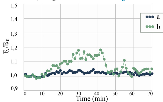
Fig. 3. Autofluorescence changes from hippocampal CA3 area, detected from nonincubated brain slices. In the first 10 min the slices were in ACSF. From the 10th to the 40th min, the ACSF medium contained rebaudioside A. Then the brain slices were exposed again to ACSF, for 30 min. Concentrations of rebaudioside A: a -0.15 mM; b -1 mM ( n = 3 ). F_A , autofluorescence, F_{A0} , basal autofluorescence.
