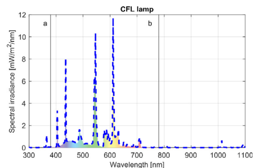
Fig. 13. CFL lamp spectrum.
