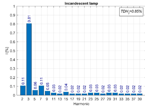
Fig. 19. Harmonic content of the halogen incandescent lamp.
