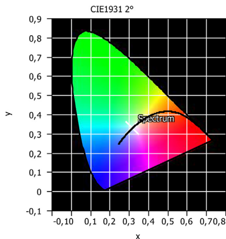
Fig. 16. Chromaticity coordinates for the LED lamp.
