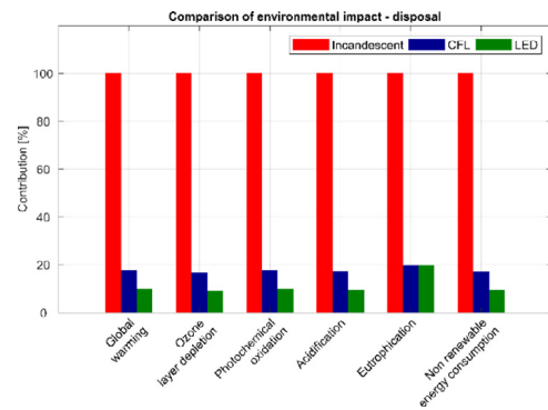
Fig. 31. Environmental impacts in the use of lamps phase.
