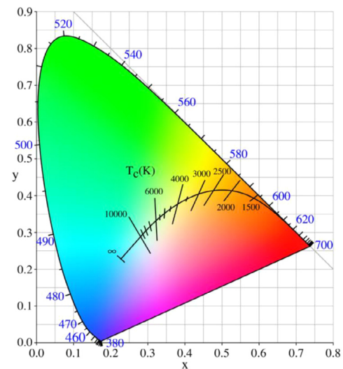
Fig. 3. Chromaticity diagram (Schanda and International Commission on Illumination, 2007).
