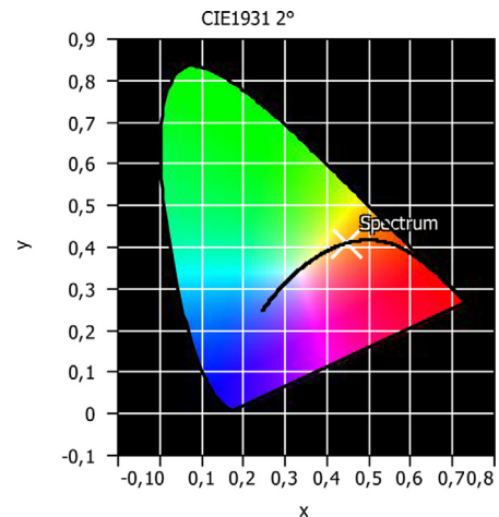
Fig. 12. Chromaticity coordinates for the halogen incandescent lamp.
