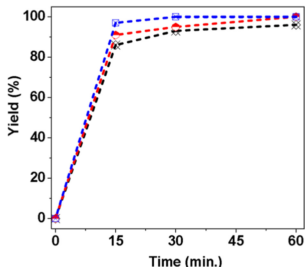
Fig. 5. The effect of the oil to methanol molar ratio: (–) black for 1:6; (–) red for 1:9 and (–) blue for 1:12. (For interpretation of the references to colour in this figure legend, the reader is referred to the web version of this article.)
