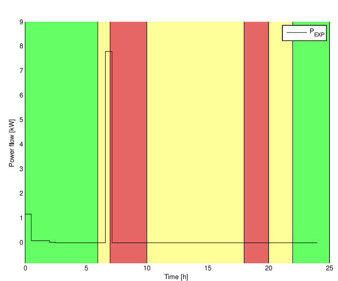
Fig. 6. Optimal power flow of exported power to the grid. (For interpretation of the references to color in this figure legend, the reader is referred to the web version of this article.)
