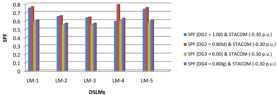
Fig. 4. SPF profiles with integration of various types of DGs (such as DG1, DG2, DG3 and DG4) and STATCOM (-0.30 p. u.) with DSLMs.
