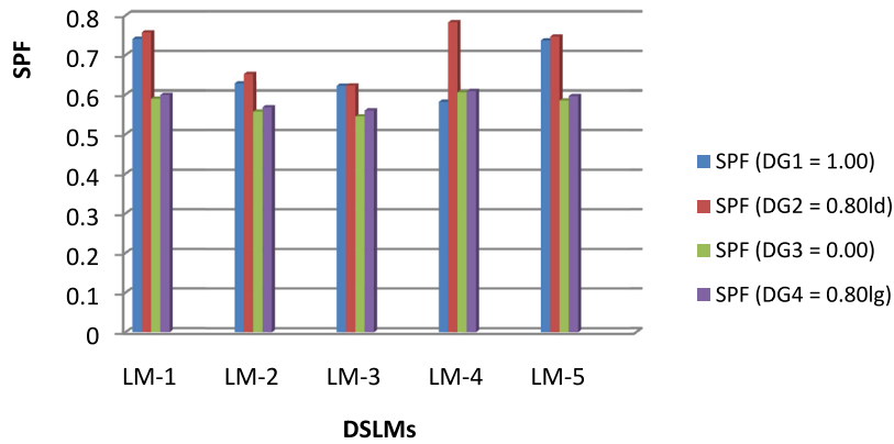
Fig. 3. SPF profiles with various types of DGs (i.e. DG1, DG2, DG3 and DG4, respectively) with DSLMs.
