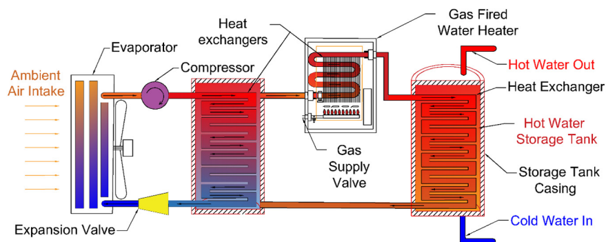
Fig. 14. Schematic diagram of the hybrid gas-fired heat pump water heater (GFHPWH).
