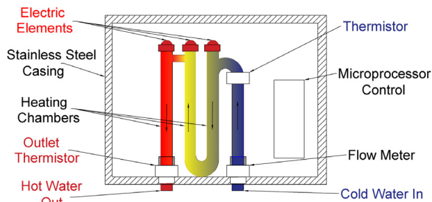
Fig. 3. Electric tankless water heater (ETWH).
