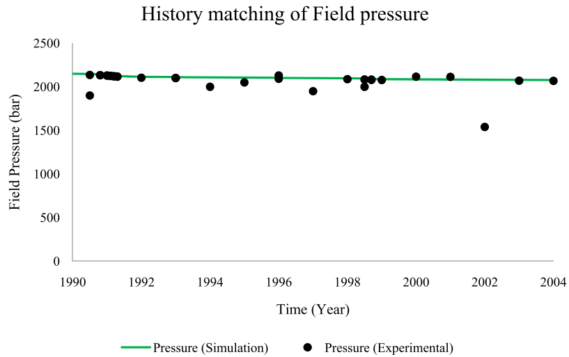
Fig. 7. History matching of field pressure.
