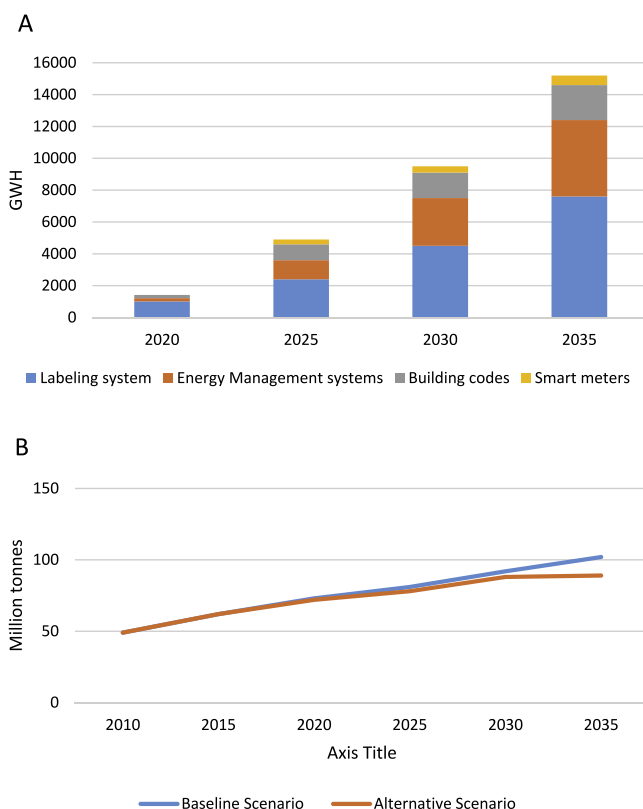
Fig. 10. Electricity savings from the introduction energy efficiency and conservation measures (A) and corresponding GHG reductions (B) (JICA, 2013).
