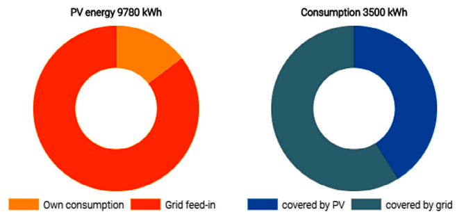
Fig. 10. Energy feed-in grid and energy consumption covered by PV and grid PV*SOL.
