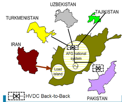
Fig. 21. Proposed regional synchronization solution (DABS, 2016b).
