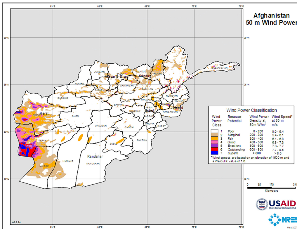
Fig. 12. Afghanistan potential wind sites map (NREL, 2007).
