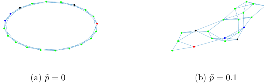
Figure 7: Watts-Strogatz small world network with N = 20 , K = 2 (the mean degree is thus 4) and wiring probabilities (a) \tilde{p} = 0 and (b) \tilde{p} = 0.1 . The color node code is: green = household; blue = school; red = hospital; black = company.
