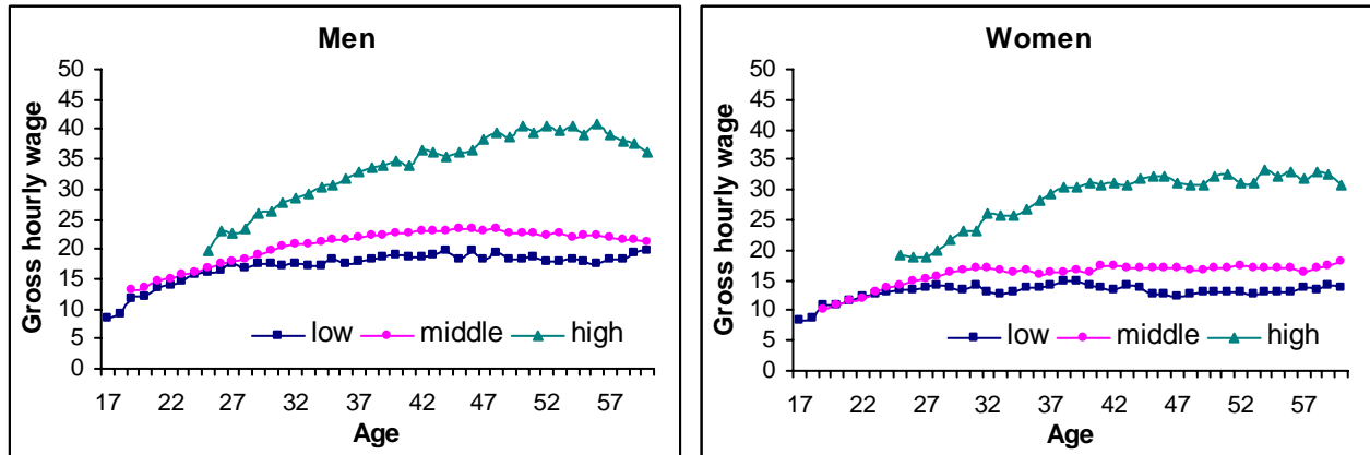
Figure 2: Age-wage profiles by qualification level (DM)
