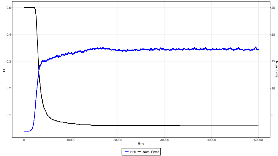
Figure 1: Time series of the Herfindahl-Hirschman index and the number of firms in the industry for the benchmark parametrization; average across 20 MonteCarlo simulations. Presence of unit root for the time series of the Herfindahl index is rejected at the 1% level by the augmented Dickey-Fuller test for the periods t \in [20001, 50000] .
