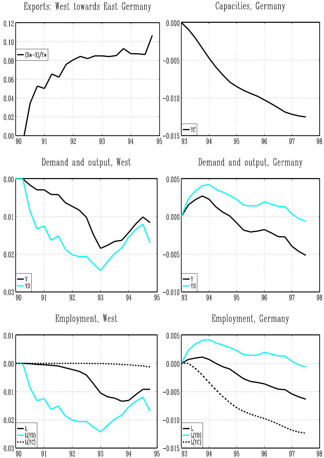
Figure 5: Simulated effects of export and fiscal policy shocks
