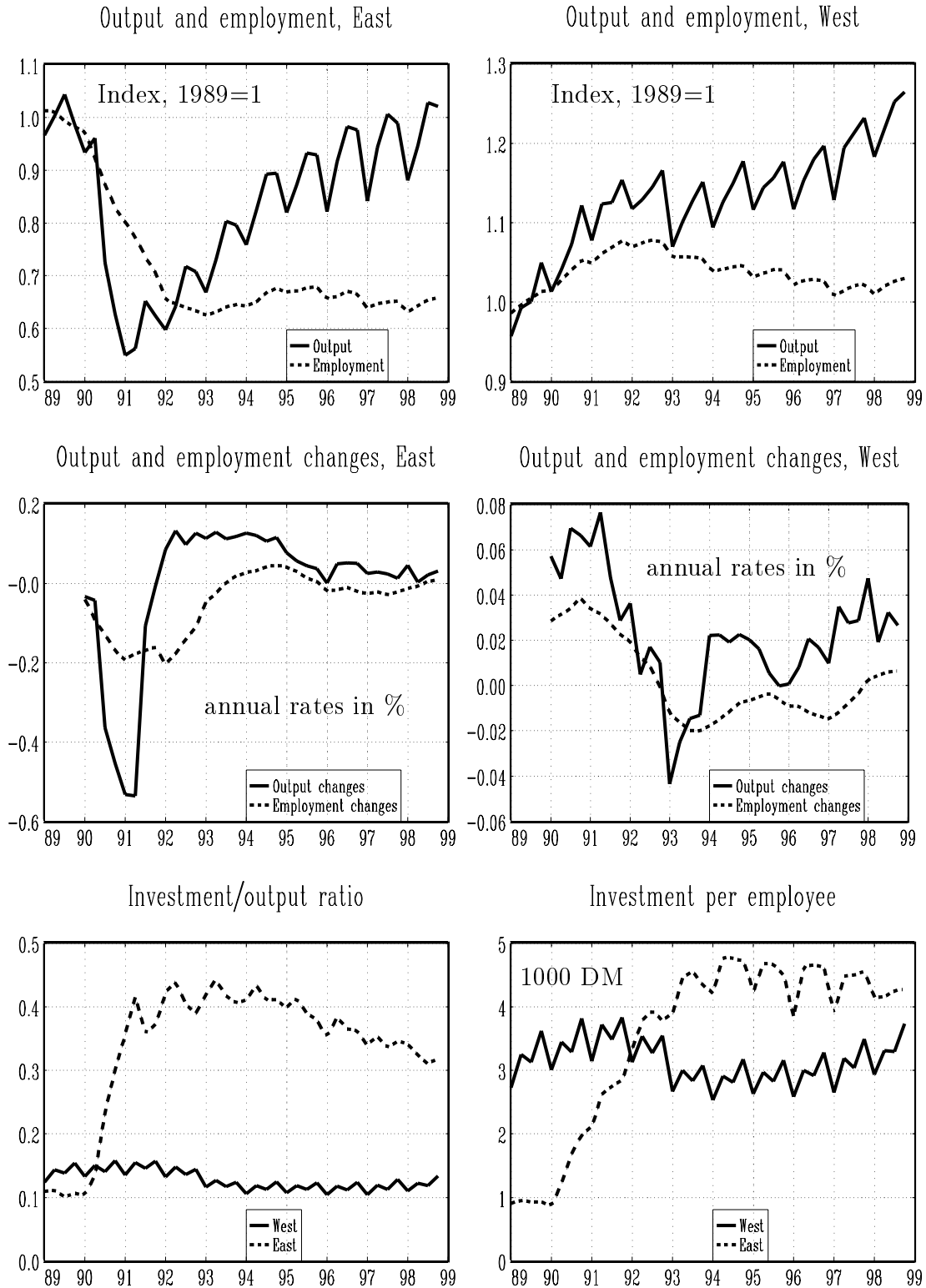
Figure 1: Output, employment and investment
