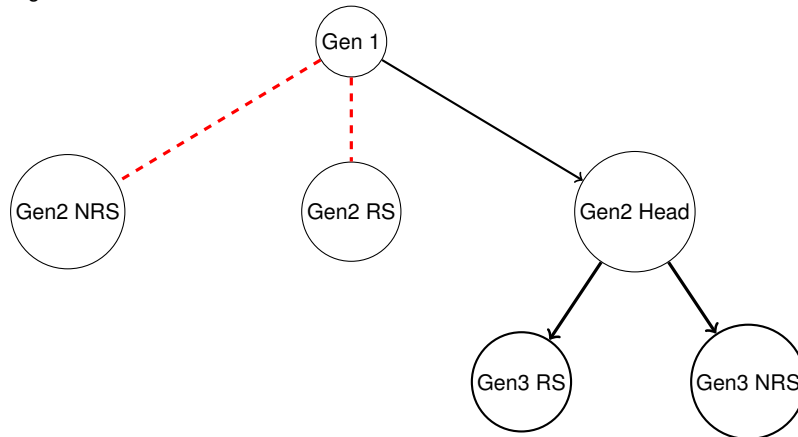
Figure 1: Generation tree
