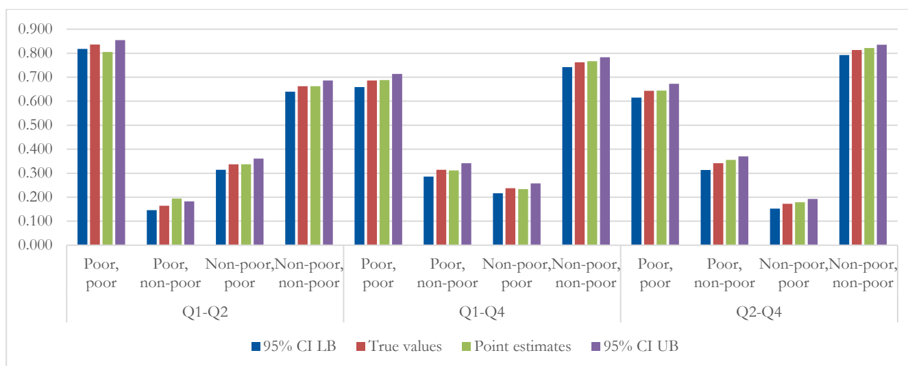
Figure 2: True transition rates (with CIs) and point estimates obtained using synthetic panels: conditional probabilities
