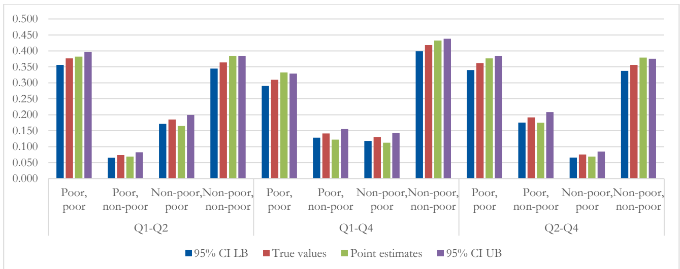
Figure 1: True transition rates (with CIs) and point estimates obtained using synthetic panels: unconditional probabilities
