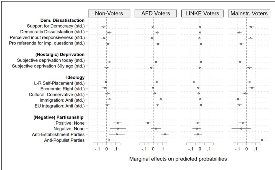
Figure 4. Extended Models for Non-Voters, AfD Voters, Die Linke Voters and Mainstream Voters.
