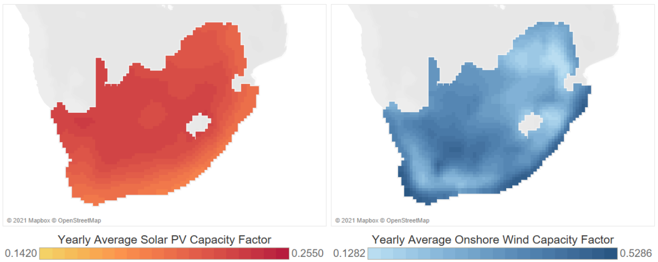
Figure 4: Presentation of the yearly average capacity factors for onshore wind and solar PV per data point in a 21x21km grid. Source: Own illustration
