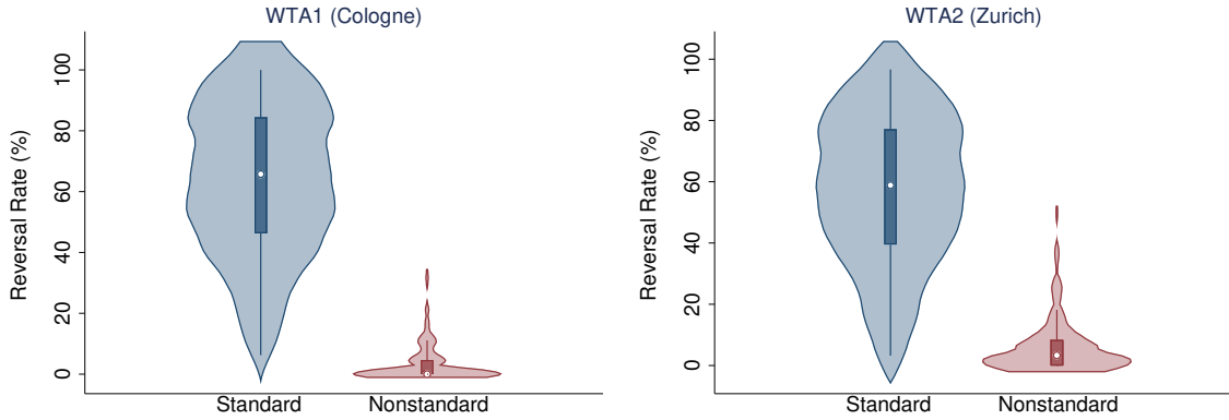
Figure 8: Reversal rates for WTA1 (left) and WTA2 (right).
