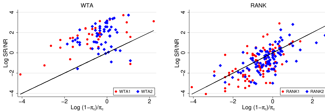
Figure 11: Figure plots individual reversal ratio \frac{SR}{NR} (on a log scale) against the individual choice odds \frac{1-\pi_c}{\pi_c} . Left: WTA1 and WTA2 . Right: RANK1 and RANK2 .
