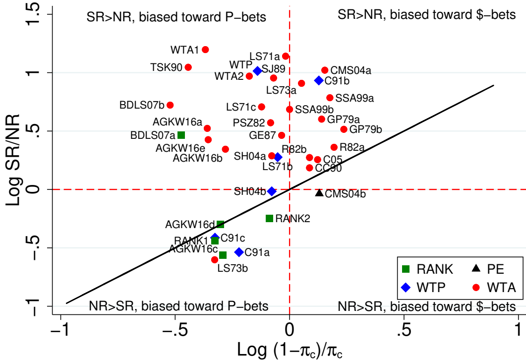
Figure 12: Logarithm of the aggregate reversal ratio \frac{SR}{NR} against logarithm of the aggregate choice odds \frac{1-\pi_c}{\pi_c} for different 28 previous experiments in the literature (see Table 2) and our five new experiments.
