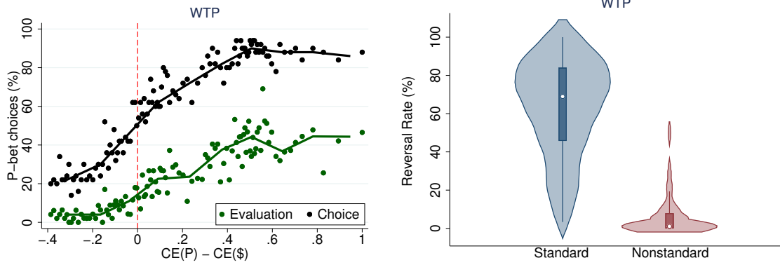
Figure A.1: Strength-of-preference effects (left) and reversal rates (right) for WTP .
