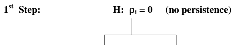
Figure 4: Sequential testing of the hypotheses
