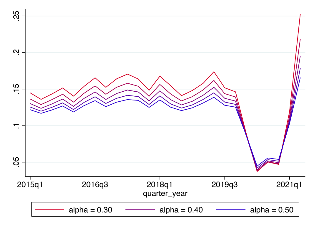
Figure 15: Aggregate JFPs for ‘typical’ values of \alpha
