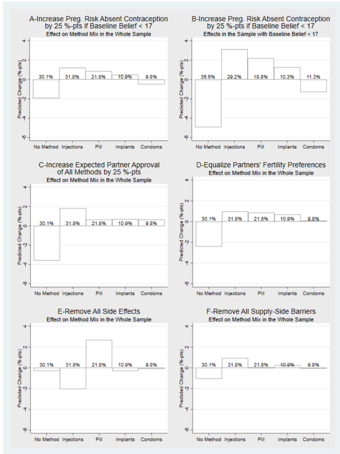
Figure 2: Counterfactuals
