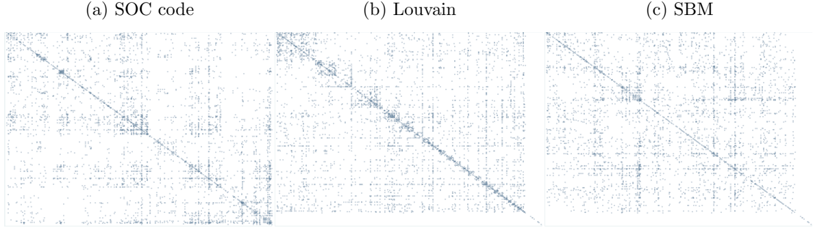
Figure 2: Voluntary occupational-mobility network adjacency matrix
