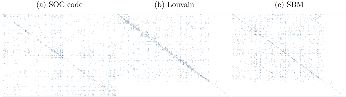
Figure 3: Involuntary occupational-mobility network adjacency matrix
