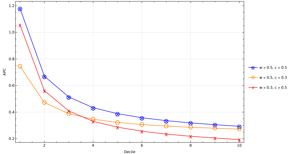
Figure 1: The figure plots the APCs per income decile for different parametrisations and with homophily strength \rho = 4 and b = 0.75 , averaged over 100 simulation runs. Lines are visual aids only.
