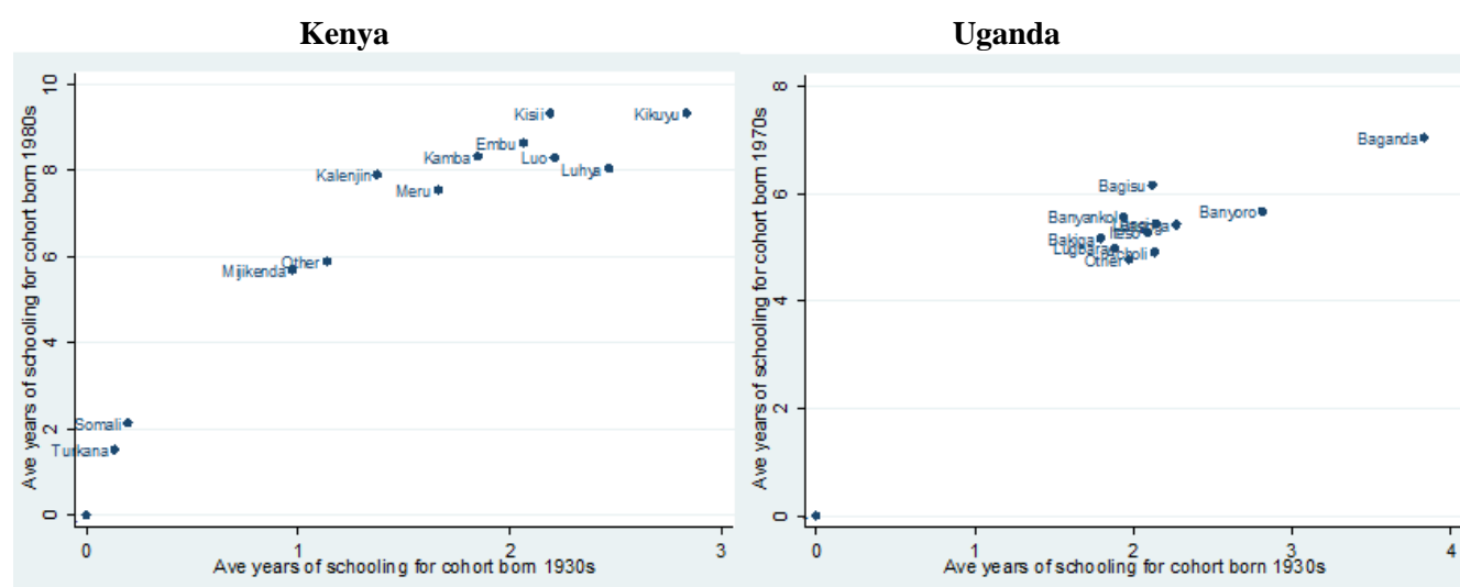
Figure 3. Correlation between average years of schooling by age cohort and ethnic group
