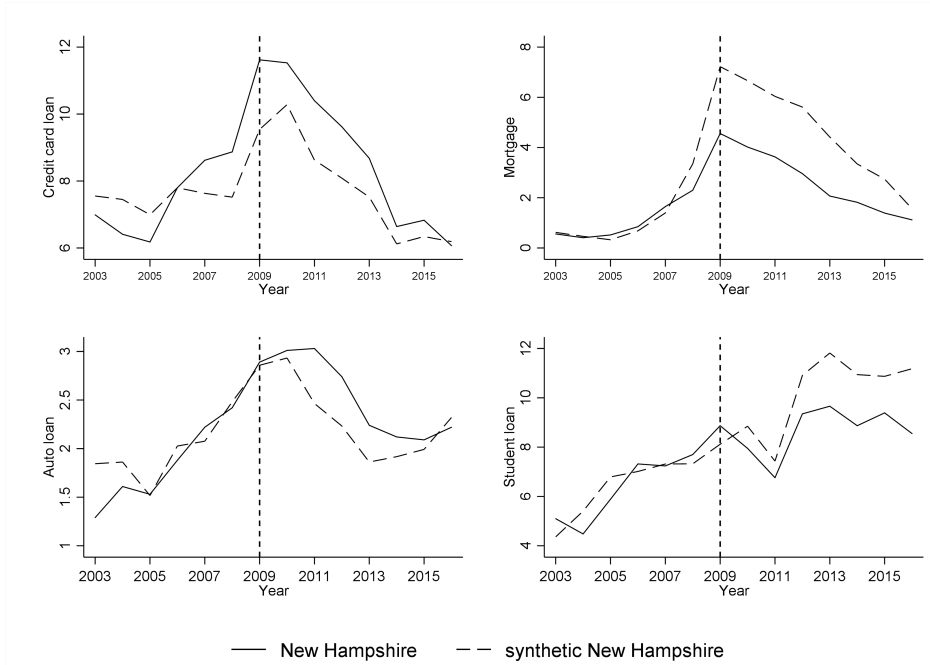
Figure 5: Visual Synthetic Control Results: New Hampshire Informal Bankruptcy
