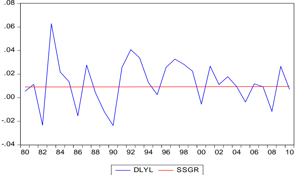
Figure 4: SSGR for Australia
