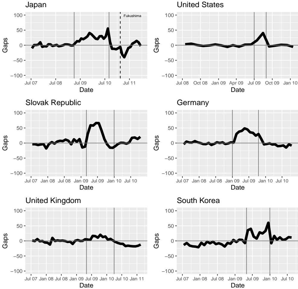
Figure 2: Gap Plots
