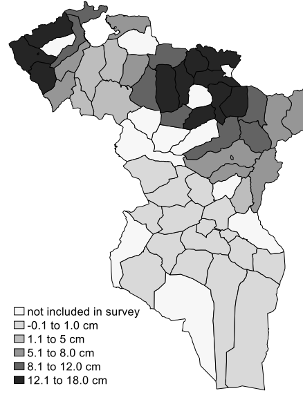
(b) Deviation in snow depth in 2009/10 winter from long-term local mean
