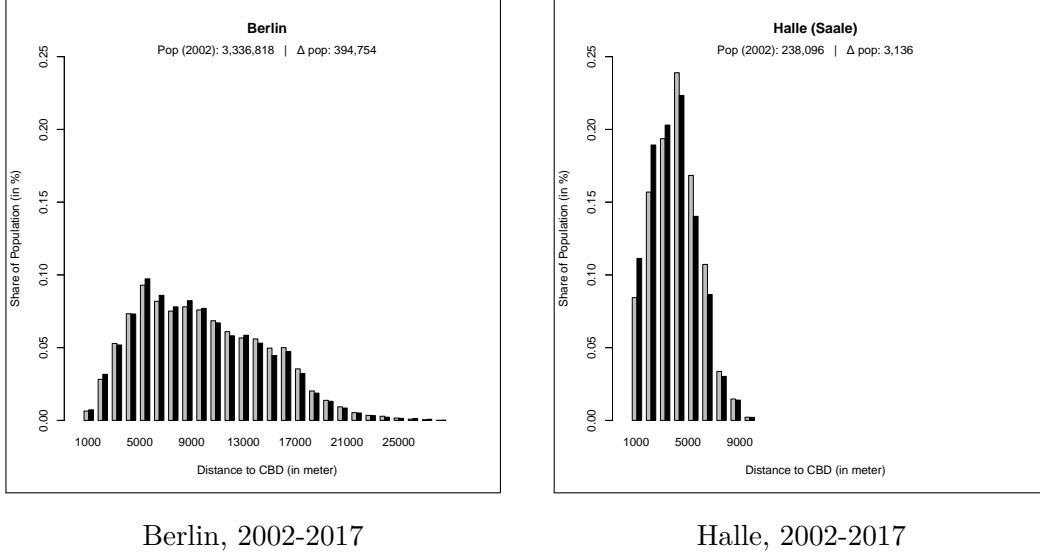
Figure 3: Two Selected Population Profiles
