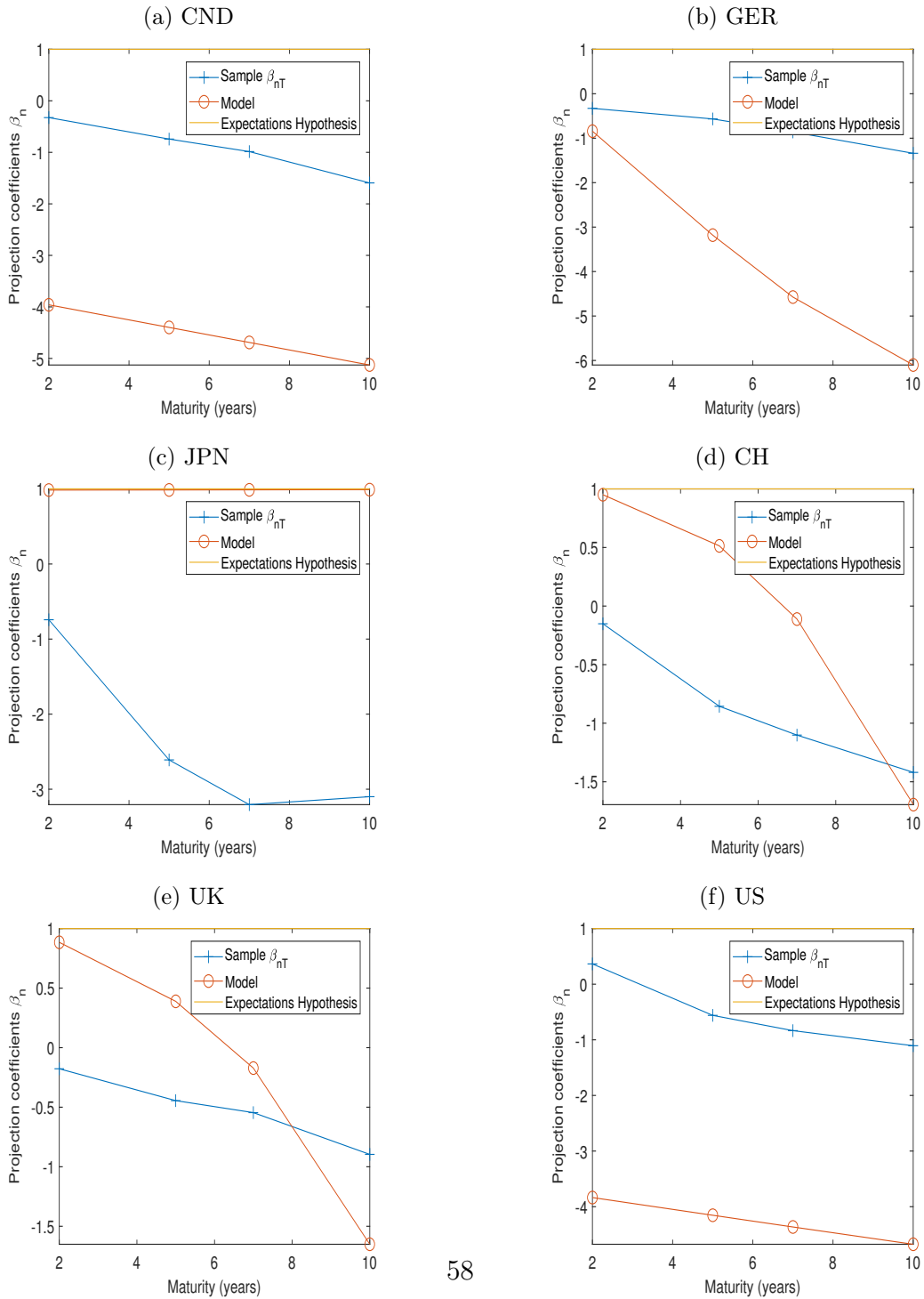
Figure 15: Testing the expectations hypothesis: Campbell-Shiller regression coefficients
