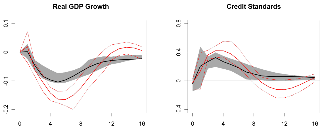
Panel A: IRFs for Shocks in the Interest Rate
