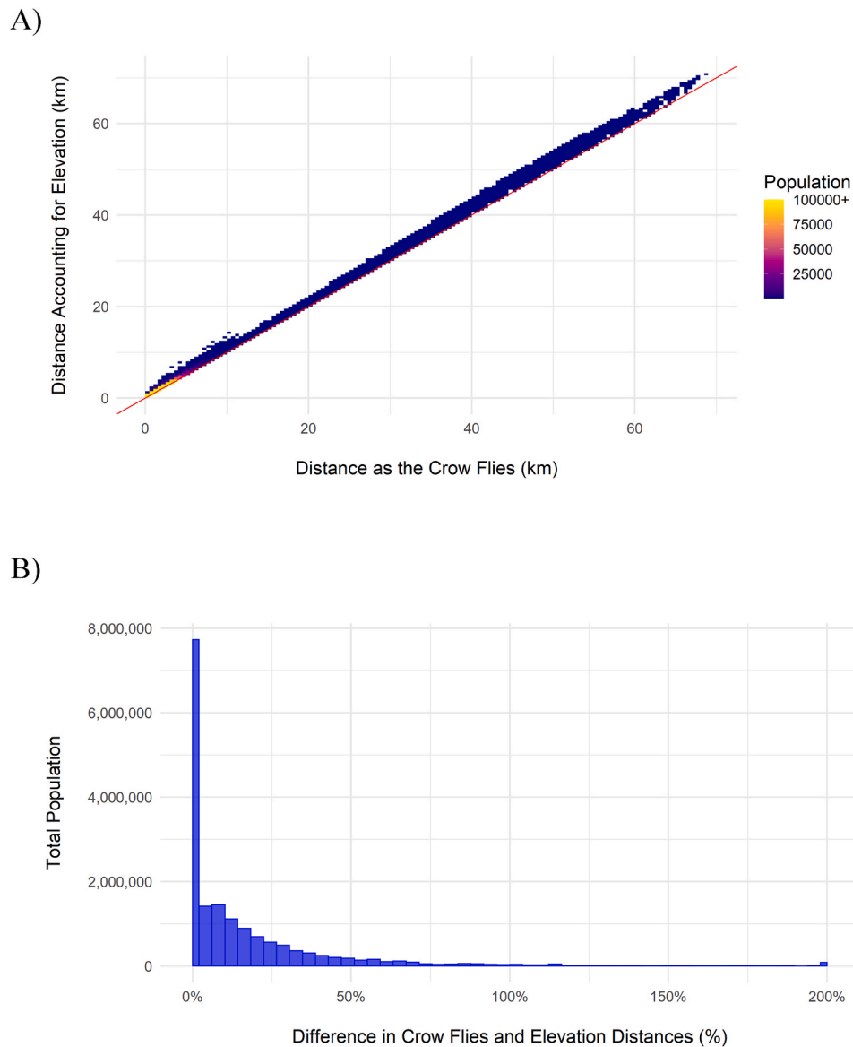
Fig. 7. (Panel B): Histogram displaying the distribution in the difference between “as-the-crow-flies” distances with distances calculated using the “path of least resistance” through elevation changes, (Panel A): Comparison of “as-the-crow-flies” distances with distances calculated using the “path of least resistance” through elevation changes, Note: Sample subsets to only public primary schools in 2017 in Guatemala.
